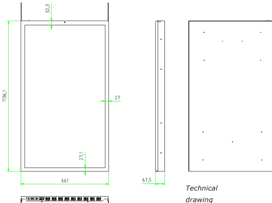
Rope suspension
