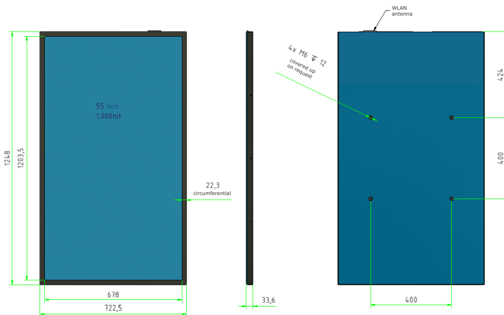
Technical drawing
